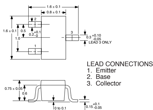
PACKAGE OUTLINE 19
