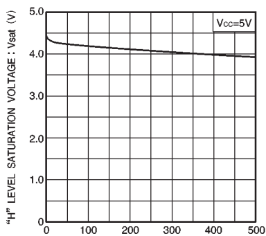
Fig.7 High level saturation voltage vs. output current
