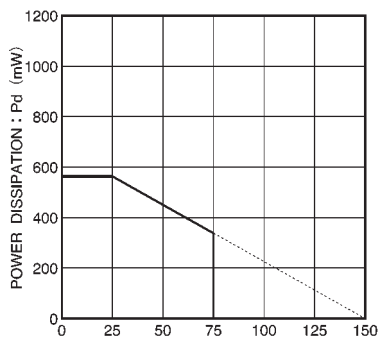
Fig.4 Power dissipation
