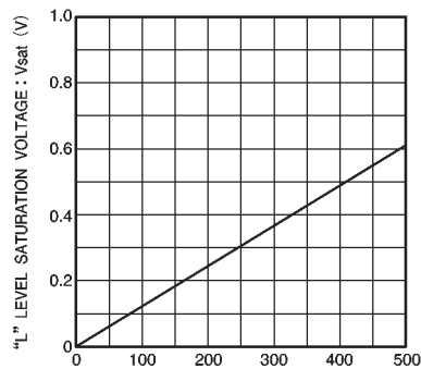
Fig.6 Low level saturation voltage vs. output current
