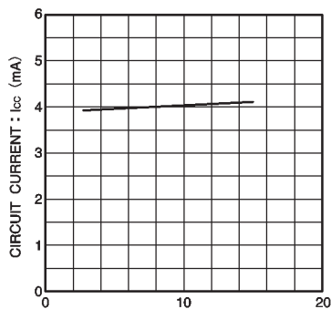
Fig.5 Circuit current vs. power supply voltage
