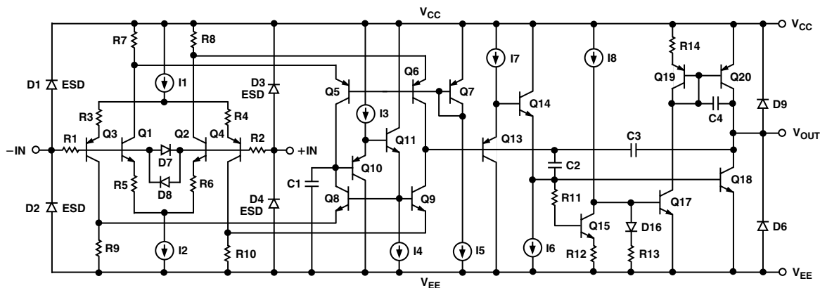
Figure 19. Simplified Schematic
