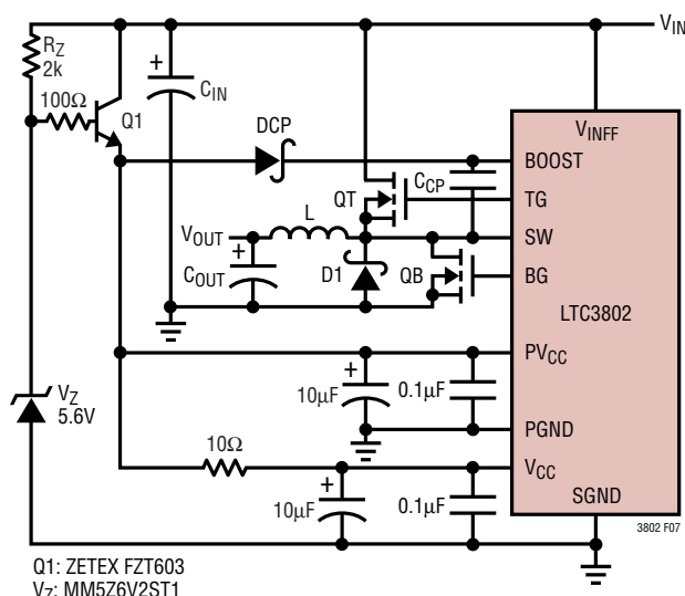
Figure 7. LTC3802 Power Supply Inputs
