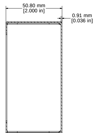
SECTION DD-DD
