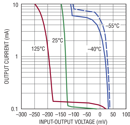
5V Minimum V_{IN} to V_{OUT} Differential (Sinking)
