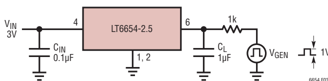
Figure 3. Load Current Response Time Test Circuit
