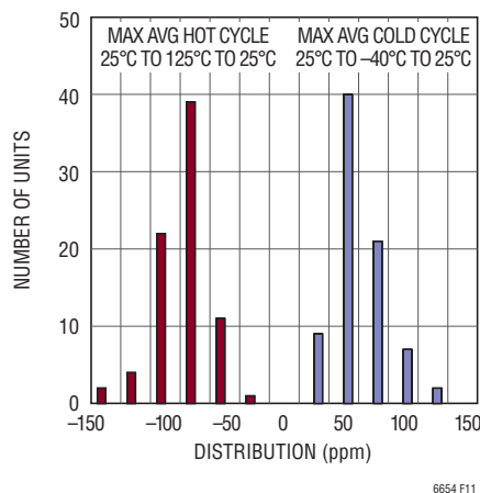
Figure 11. Thermal Hysteresis -40°C to 125°C
