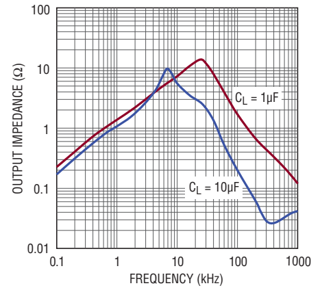
5V Output Impedance vs Frequency
