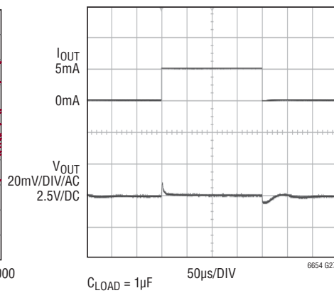
2.5V Load Transient Response (Sinking)
