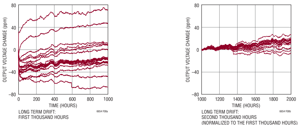
Figure 8. LT6654-2.5 Long Term Drift
