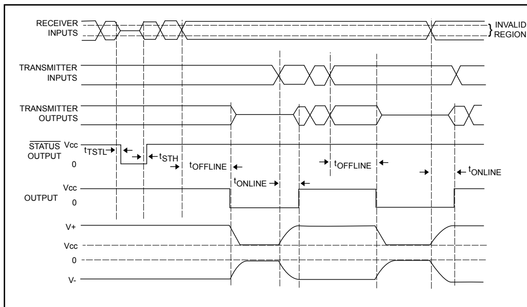
Auto On-Line® Plus Timing Diagram
