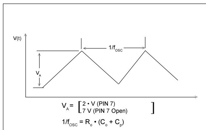
Fig. 6b: Oscillator Waveform Diagram
