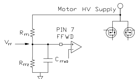
Fig. 7 Feedforward Connection Diagram
