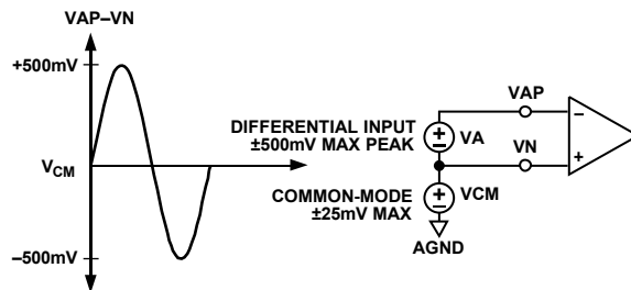
Figure 15. Maximum Signal Levels, Voltage Channel
