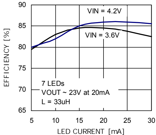
7 LED Efficiency vs. Load Current
