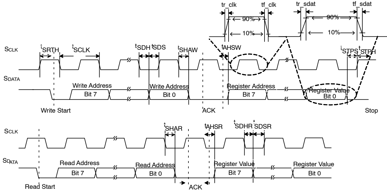
Figure 28. Two-Wire Serial Bus Timing Parameters
