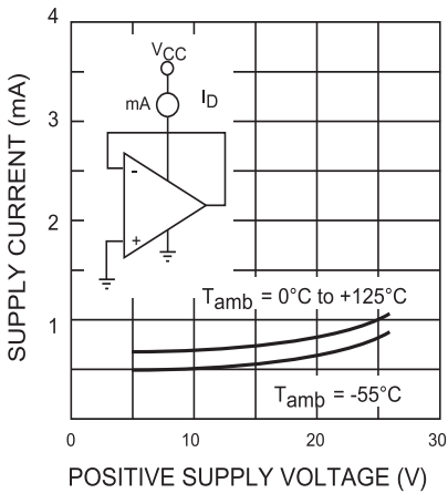
Figure 12. Supply current
