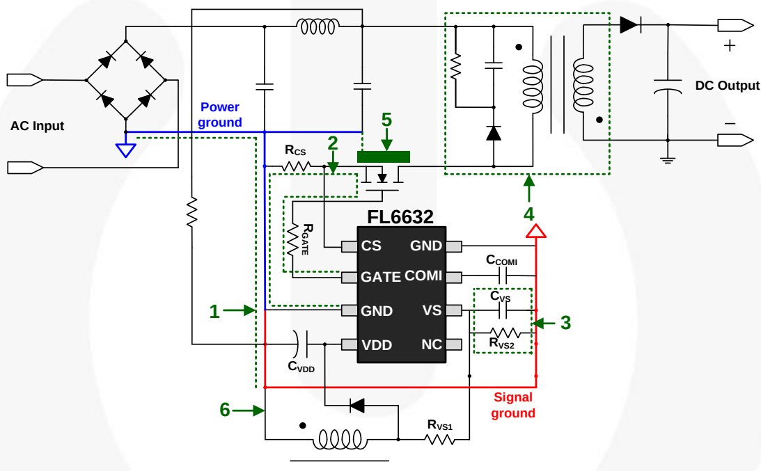
Figure 23. Layout Example
