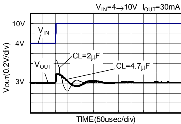
Load dependencies of overshoot
