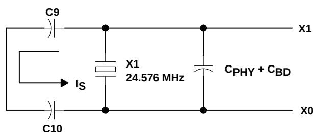
Figure 8–4. Load Capacitance for the TSB43AA22 PHY
