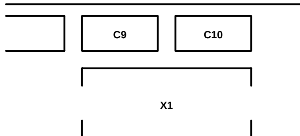
Figure 8–5. Recommended Crystal and Capacitor Layout
