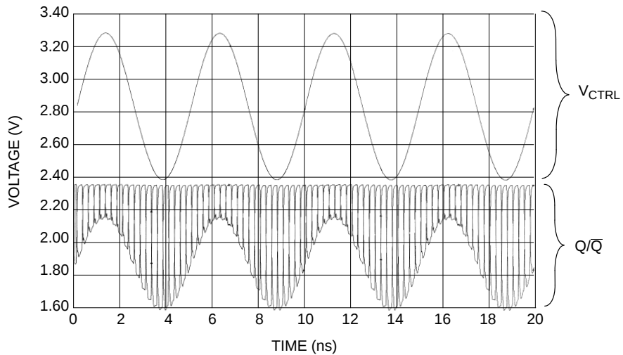
Figure 6. Output Response Under Amplitude Modulation of V_{CTRL} (Conditions Include V_{CC} - V_{EE} = 3.3 V at 25°C, f_{IN}(V_{CTRL}) = 200 MHz, and f_{IN}(D, \bar{D}) = 2 GHz)
