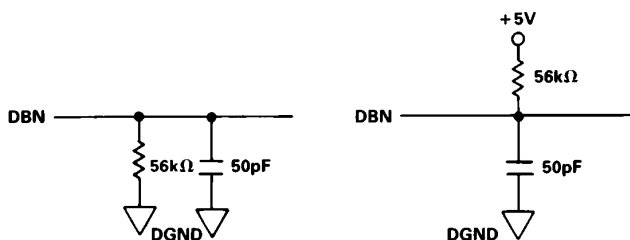
a. High-Z to V_{OH} b. High-Z to V_{OL} Figure 1. Load Circuits for Access Time
