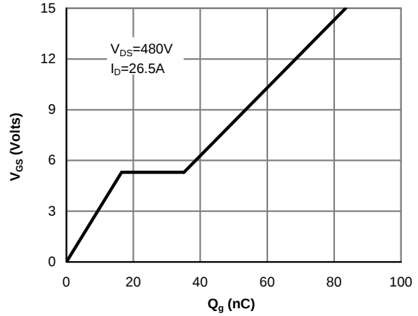
Figure 8: Gate-Charge Characteristics
