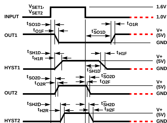
FIGURE 8. SWITCHING WAVEFORMS
