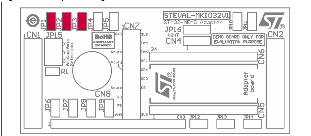
Figure 6. Setup for analog MEMS
