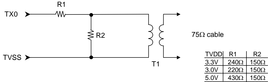
Figure 23. TX0 External Resistor Network 1
