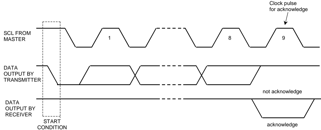
Figure 43. Acknowledge on the I 2 C-bus
