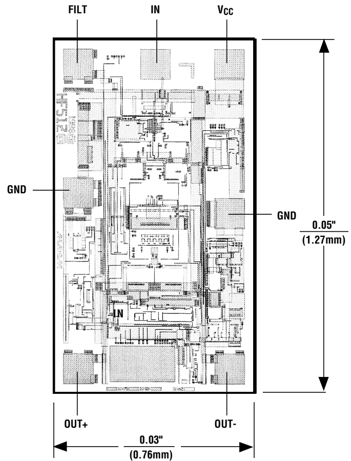
Chip Topography
