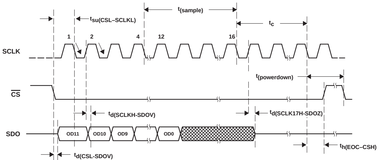
Figure 7. Critical Timing TLC2551 (FS = 1)
