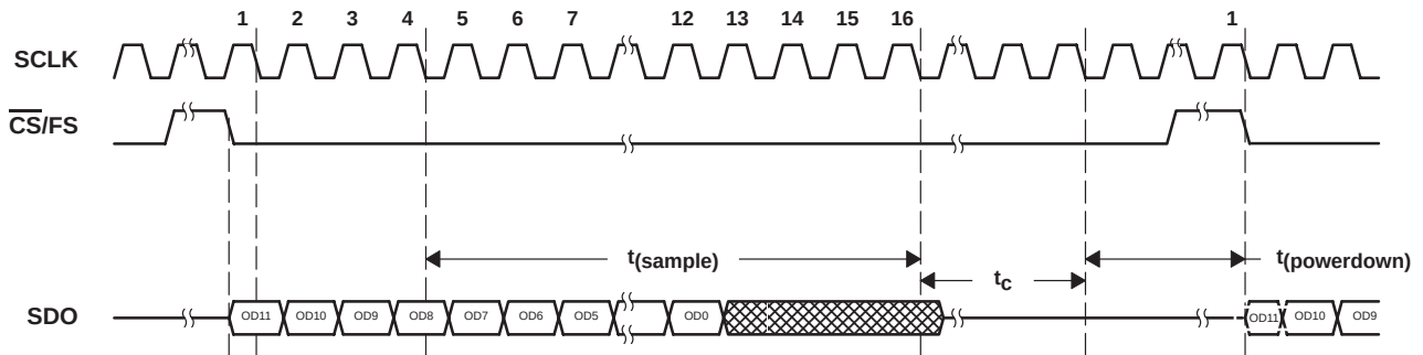
Figure 5. TLC2555 Timing
