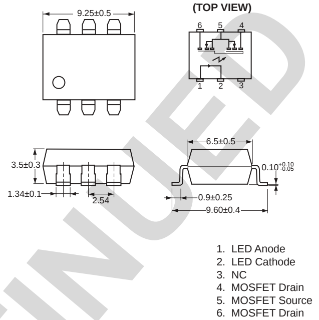
PS7122L-1A
