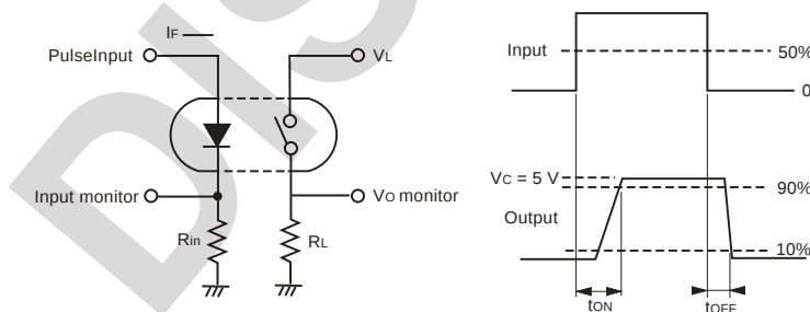
PS7122-1A, PS7122L-1A
