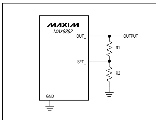
Figure 2. Adjustable Output Voltage
