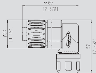
Female Cable Connector, right-angled
