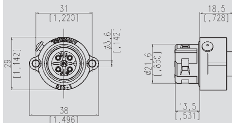
Female Receptacle
