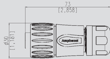
Female Cable Connector
