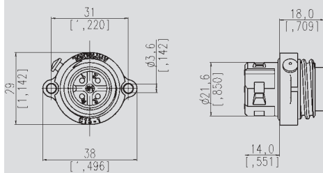
Male Receptacle
