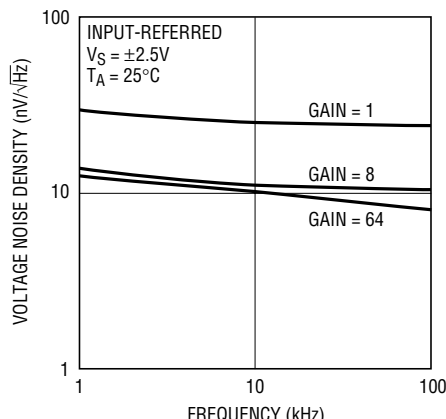
LTC6910-2 Noise Density vs Frequency
