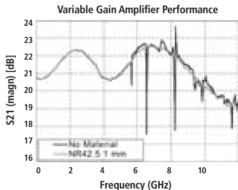
Figure 4. Performance of amplifier inside enclosure showing performance of Absorber Material (PN 2238)
