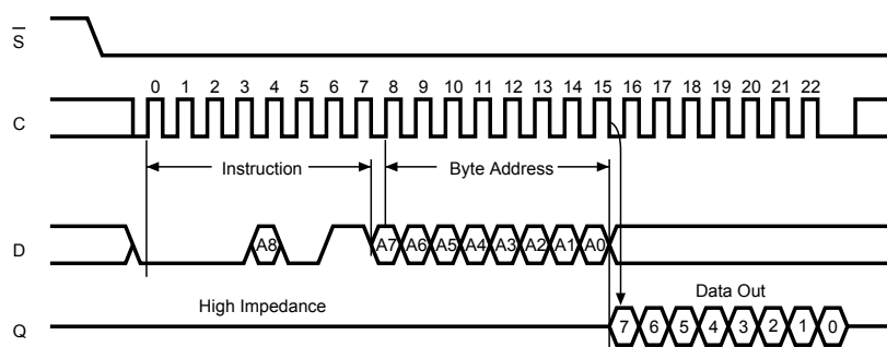
Figure 11. Read from memory array (READ) sequence
