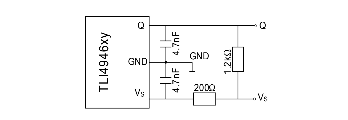
Figure 5 Application circuit
