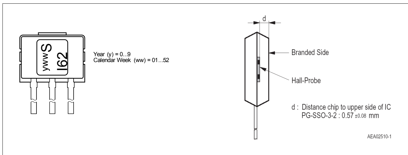
Figure 10 Marking of the TLI4946-2L and distance of the chip to the upper side
