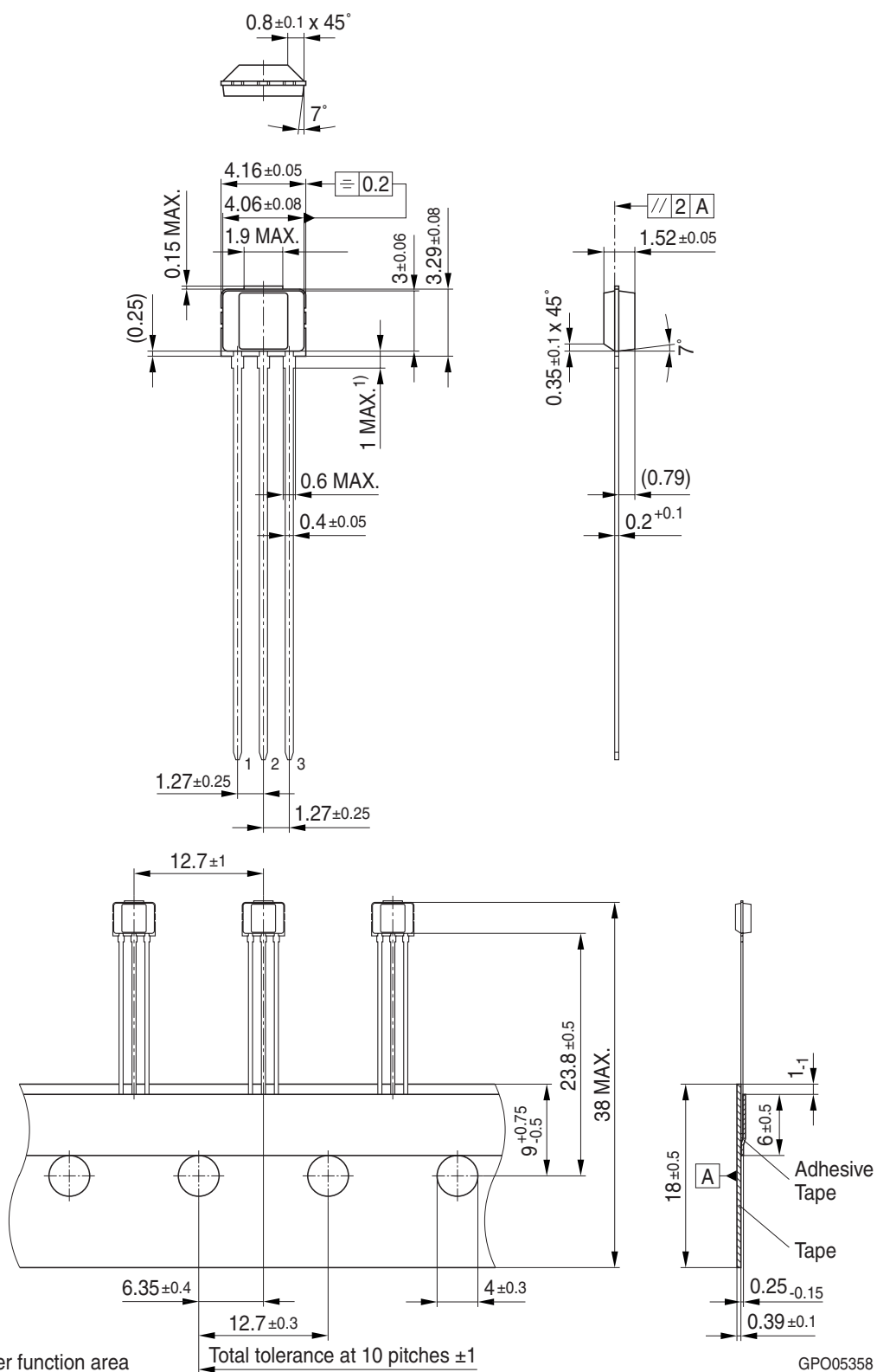
Figure 11 PG-SSO-3-2 Package Outline
