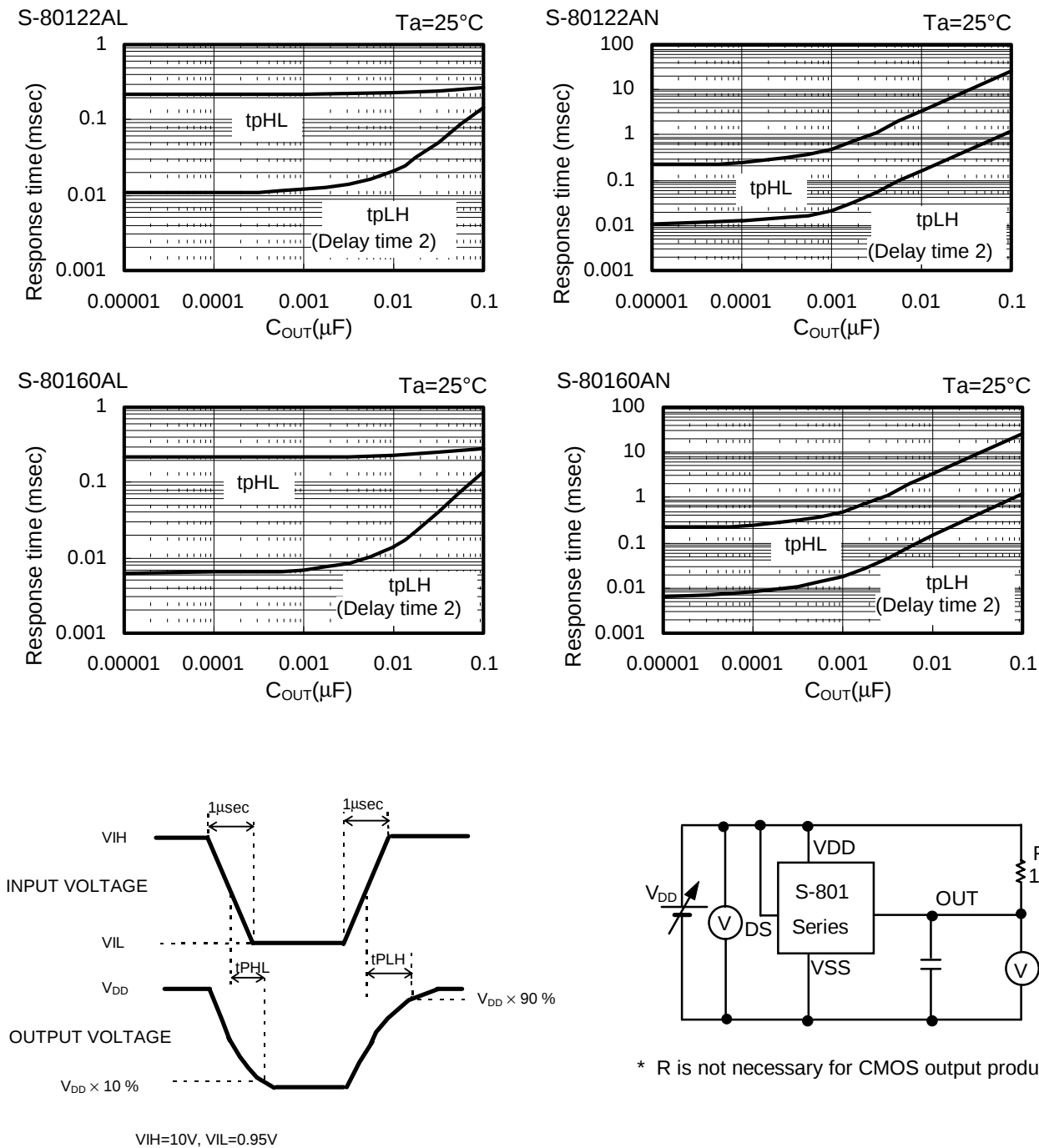
Figure 15 Measuring Conditions of Response Time
