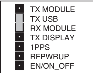
Figure 5: Jumper Configuration
