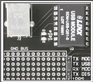
Figure 4: The USB Section
