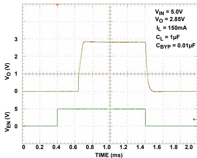
FIGURE 13. TURN ON/TURN OFF RESPONSE
