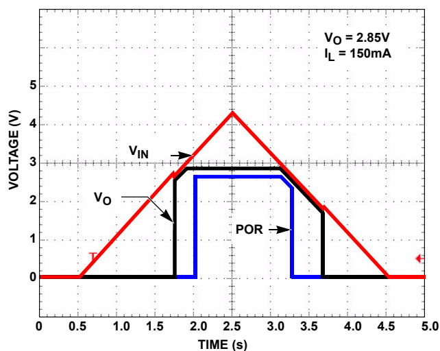
FIGURE 12. POWER-UP/POWER-DOWN
