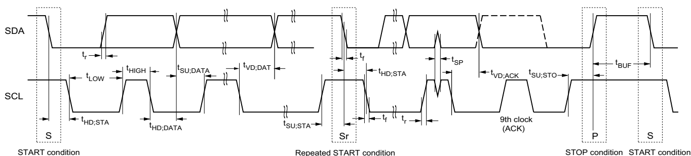
Figure 30. Timing Diagram
