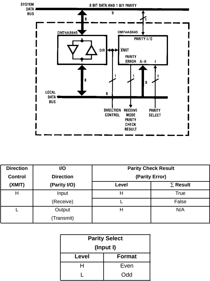
FIGURE 2. Bus I/O Parity Implementation
