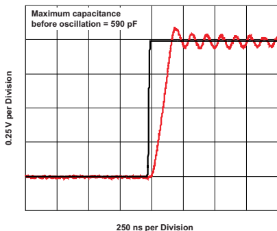
Figure 42. Pulse Response ( R_L = 10\ \text{k}\Omega , C_L = 590\ \text{pF} )
