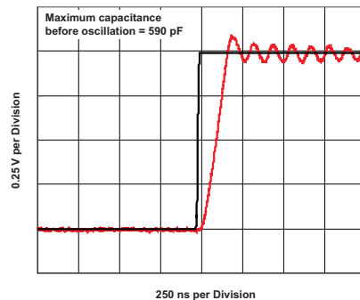
Figure 41. Pulse Response ( R_L = 2\ \text{k}\Omega , C_L = 560\ \text{pF} )
