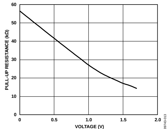
Figure 14. Digital Input Pin Pull-Up Resistance Value vs. Voltage Applied to Digital Pin, T A = 25°C, IOVDD = 1.8 V
