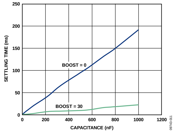
Figure 12. VBIAS Output Settling Time vs. Load Capacitance, T A = 25°C, IOVDD and AVDD = 3.3 V
