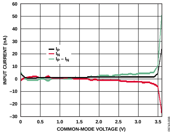
Figure 9. Input Current vs. Common-Mode Voltage (V CM ), Gain = 4, ADC Input = 250 mV, AVDD = 3.6 V, T A = 25°C, V CM = ((AIN+) + (AIN-))/2
