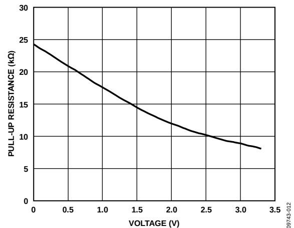
Figure 13. Digital Input Pin Pull-Up Resistance Value vs. Voltage Applied to Digital Pin, T A = 25°C, IOVDD = 3.4 V
