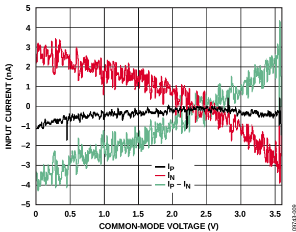
Figure 10. Input Current vs. Common-Mode Voltage (V CM ), Gain = 128, ADC Input = 7.8125 mV, AVDD = 3.6 V, T A = 25°C, V CM = ((AIN+) + (AIN-))/2
