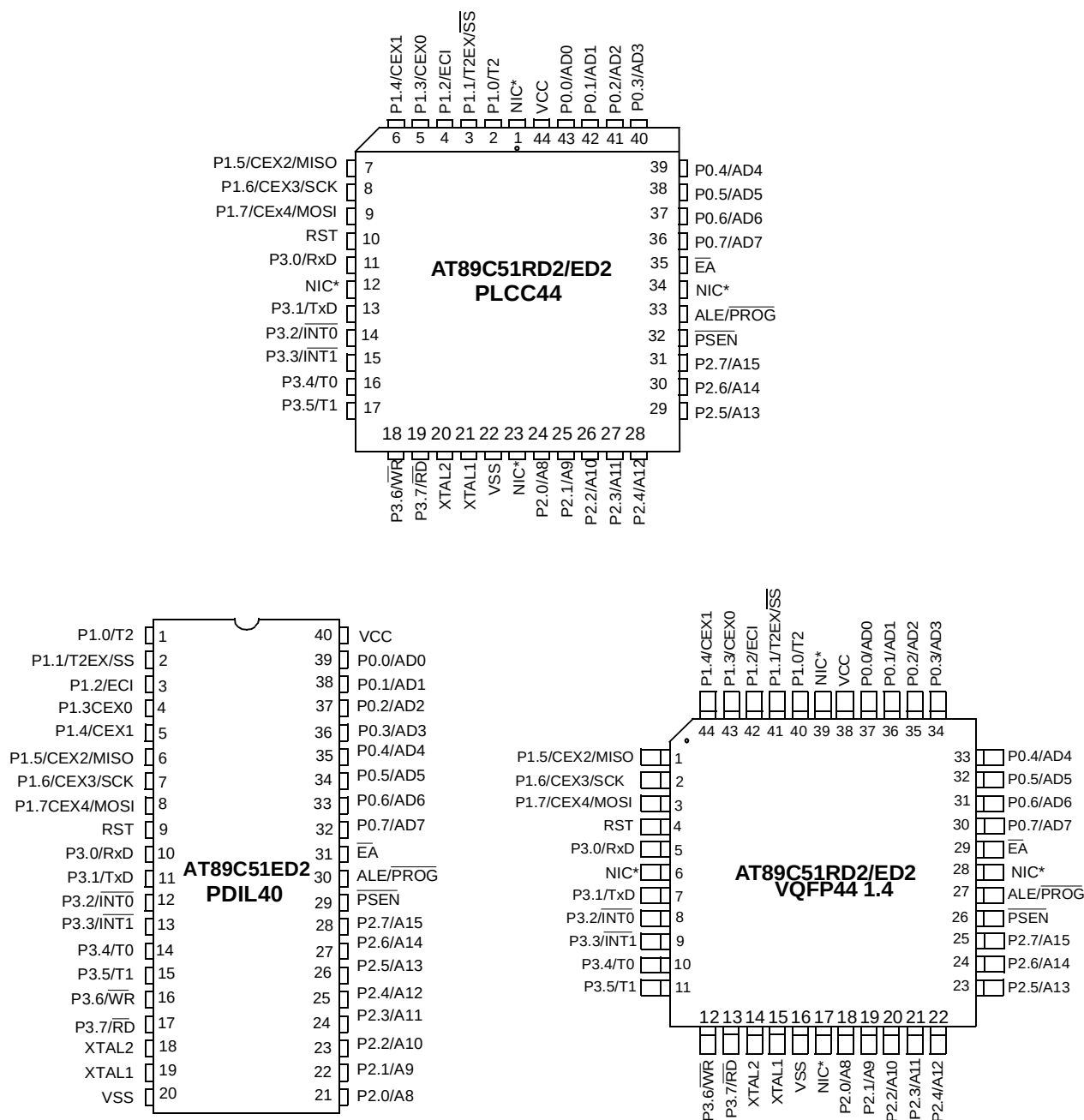
Figure 2. Pin Configurations
