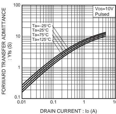
Fig.12 Forward Transfer Admittance vs. Drain current
