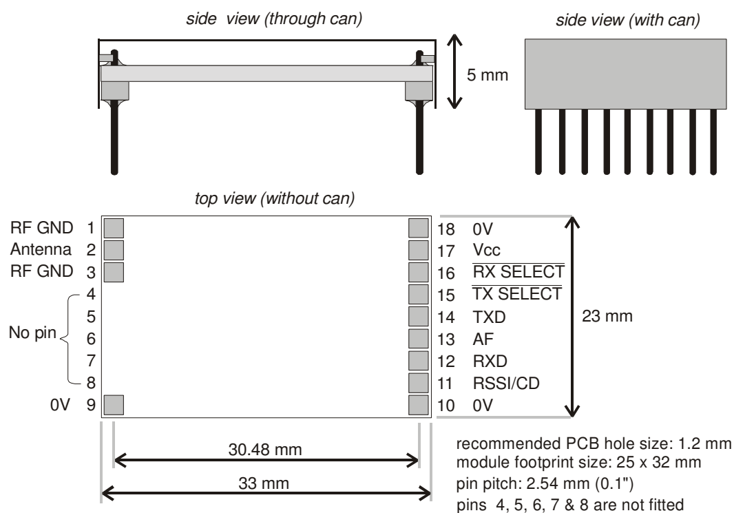
Fig. 3: Physical dimensions
