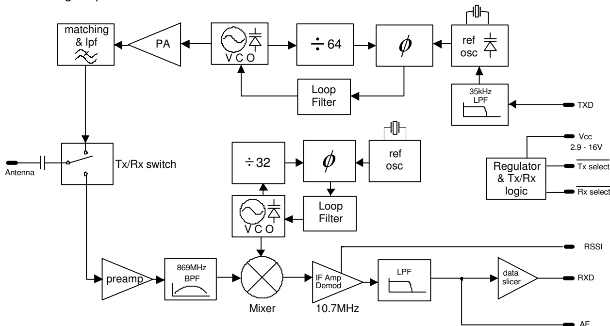
Fig. 2: Block diagram
