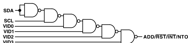
Figure 14. NAND Tree
