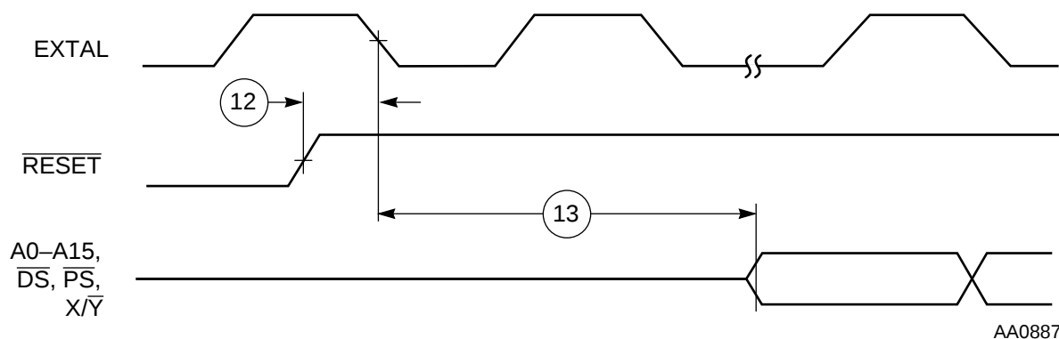
Figure 2-5 Synchronous Reset Timing
