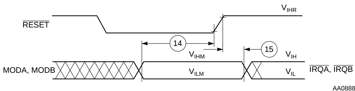
Figure 2-6 Operating Mode Select Timing
