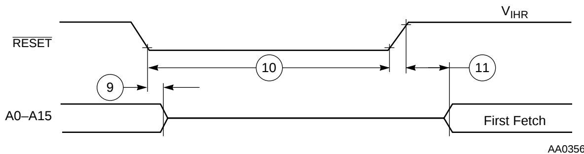
Figure 2-4 Reset Timing
