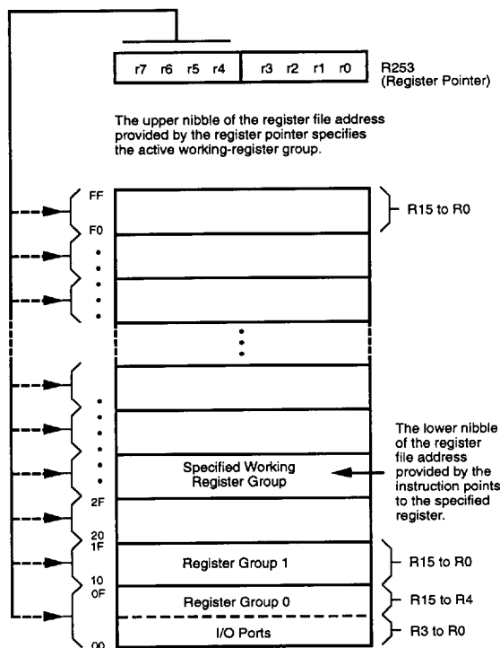
Figure 12. Register Pointer
