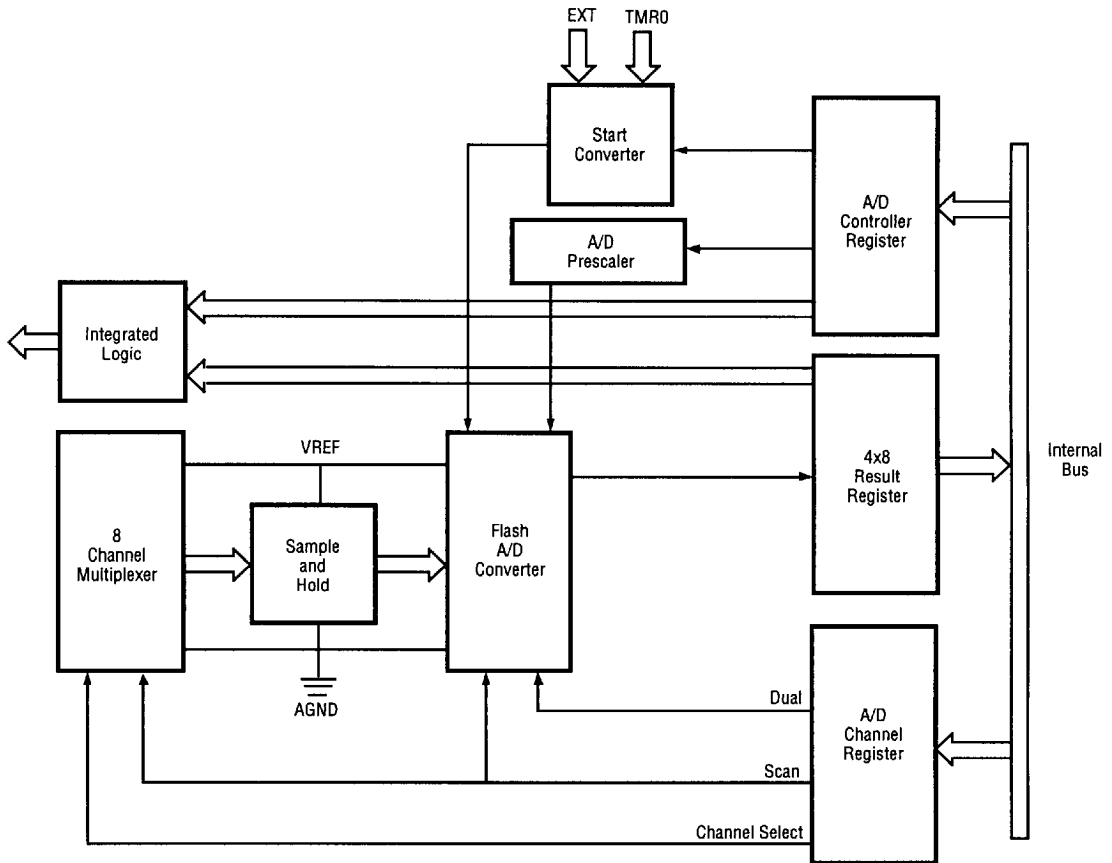
Figure 29. ADC Architecture
