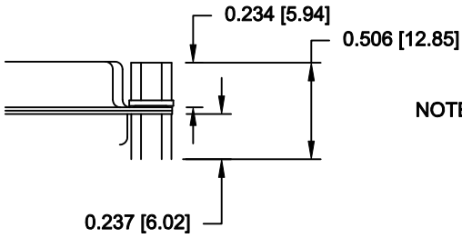
92X ..... 0.237" BOARD SIDE 0.197 MATING SIDE CN10-237-093/SFSO4404
