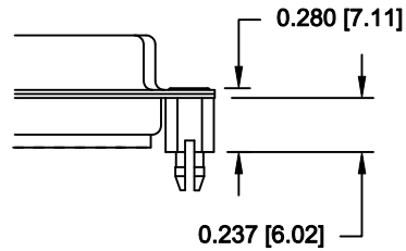
90X ..... 0.237" (BOARD SIDE) - CN10-237-093
