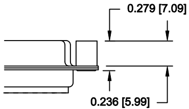
03X..... 0.236" (MATING SIDE) - CN8
