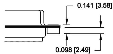
05X ..... 0.237" (BOARD SIDE) - CN10
