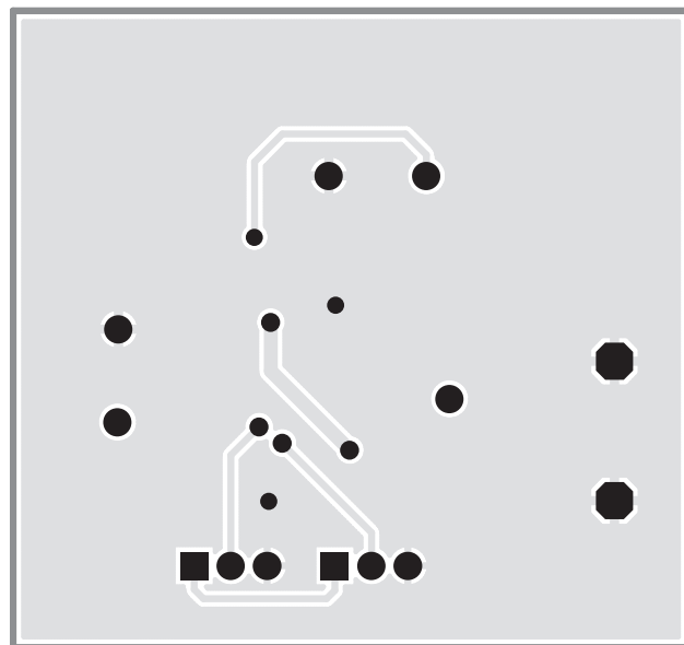
Figure 4: AAT1230/1230-1 Evaluation Board Bottom Side.
