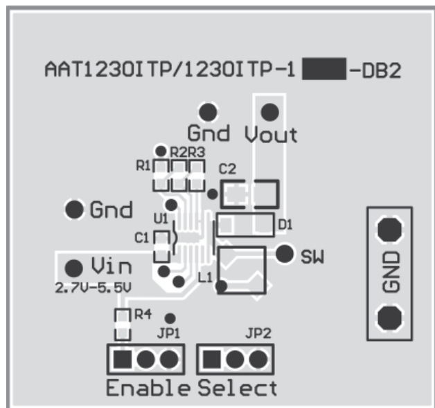
Figure 3: AAT1230/1230-1 Evaluation Board Top Side.
