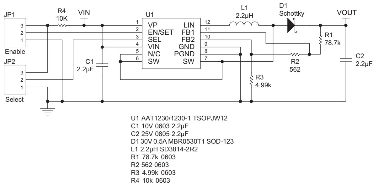
Figure 1: AAT1230/1230-1 Demo Board Schematic.
