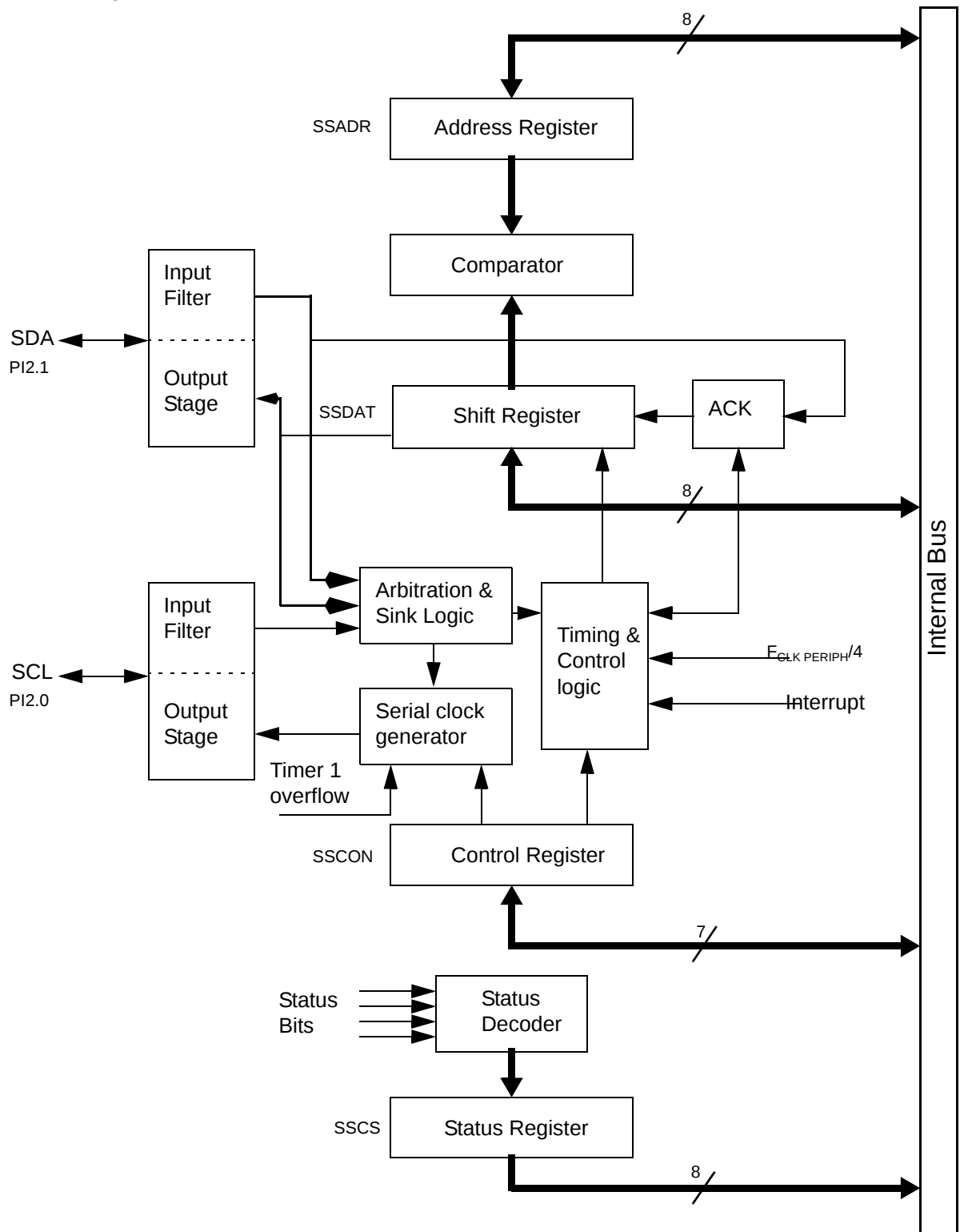
Figure 30. Block Diagram
