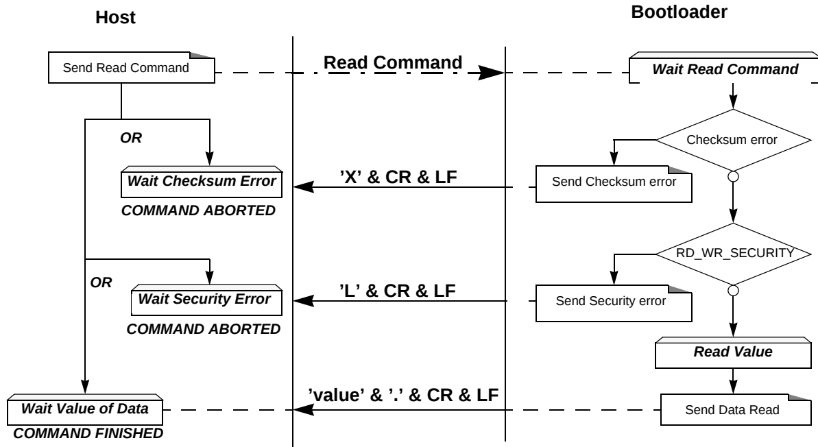
Figure 56. Read Flow
