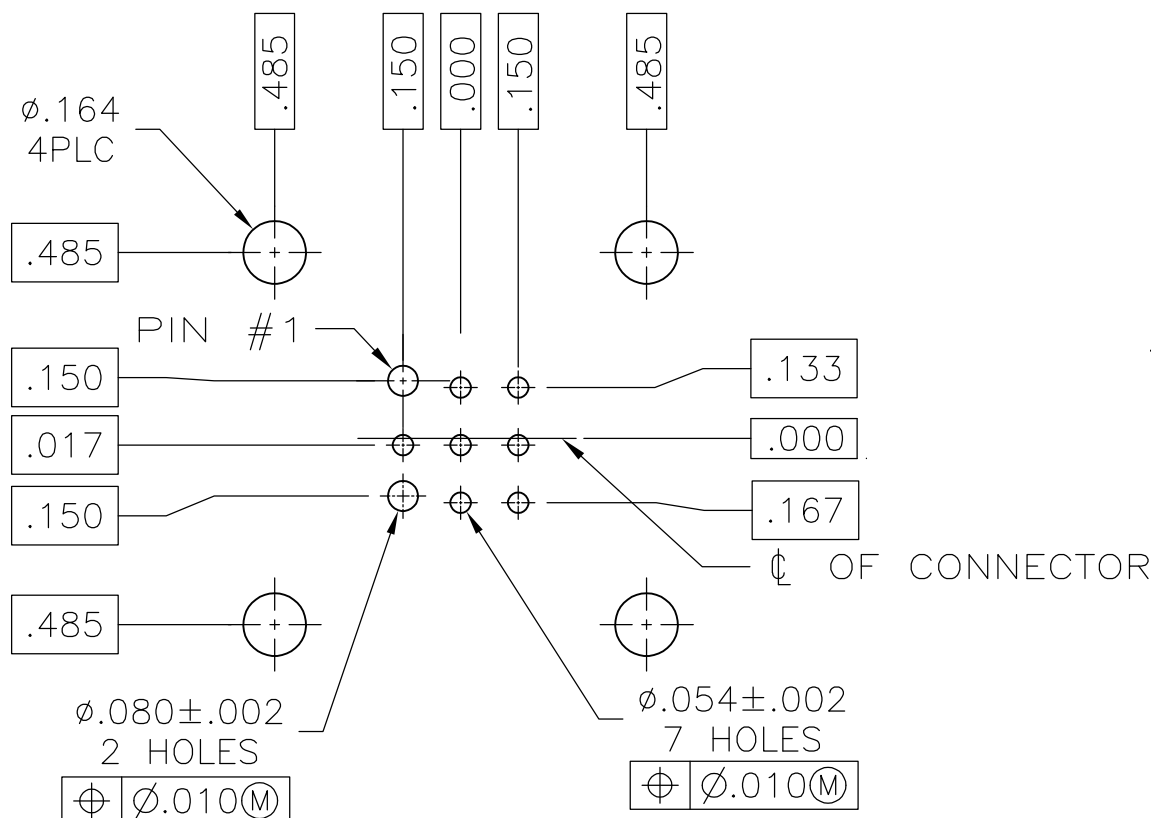
RECOMMENDED P.C. BOARD LAYOUT (1-208223-2 ONLY)
