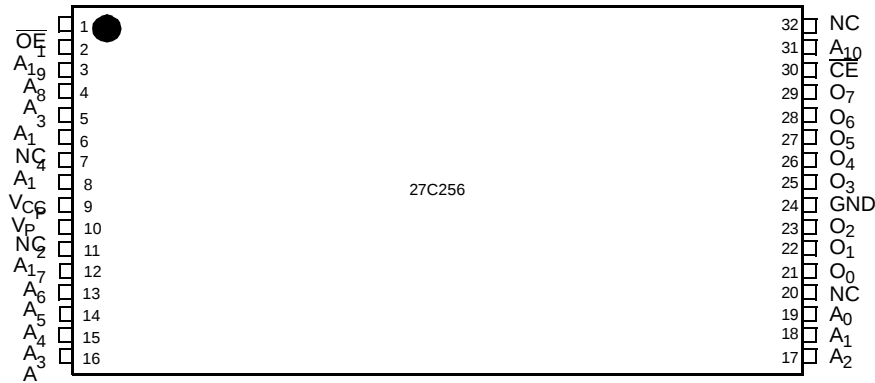
32-Pin TSOP Top View
