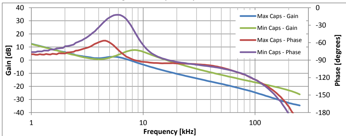
Figure 4-37 Open Loop Bode Plots
