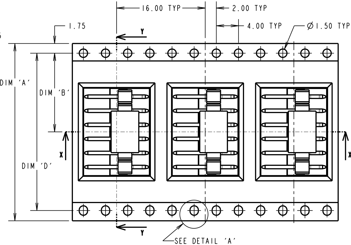
SECTION Y-Y
