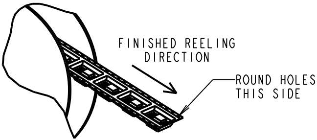
SECTION X-X
