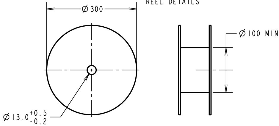
REEL DETAILS
